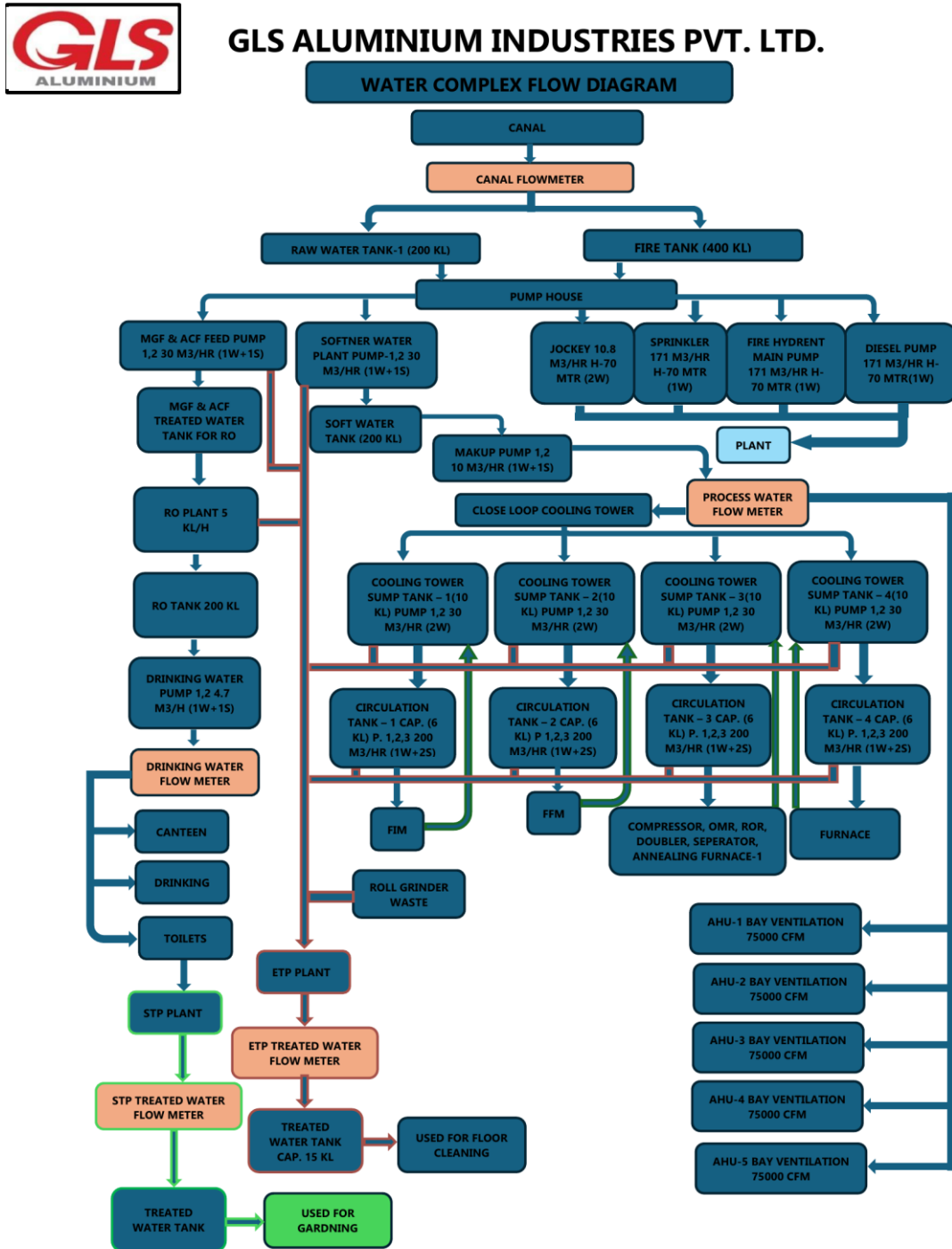
Figure 1. Water Complex Flow Diagram provided for the GLS water-management study.
